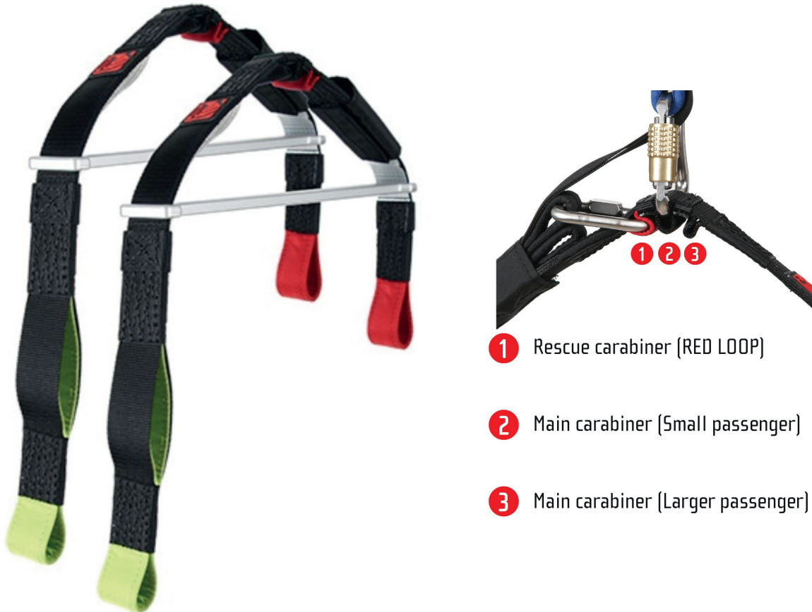
Figure: Rigid 30 mm spreader bars (hard) for Yeti Tandem 3
