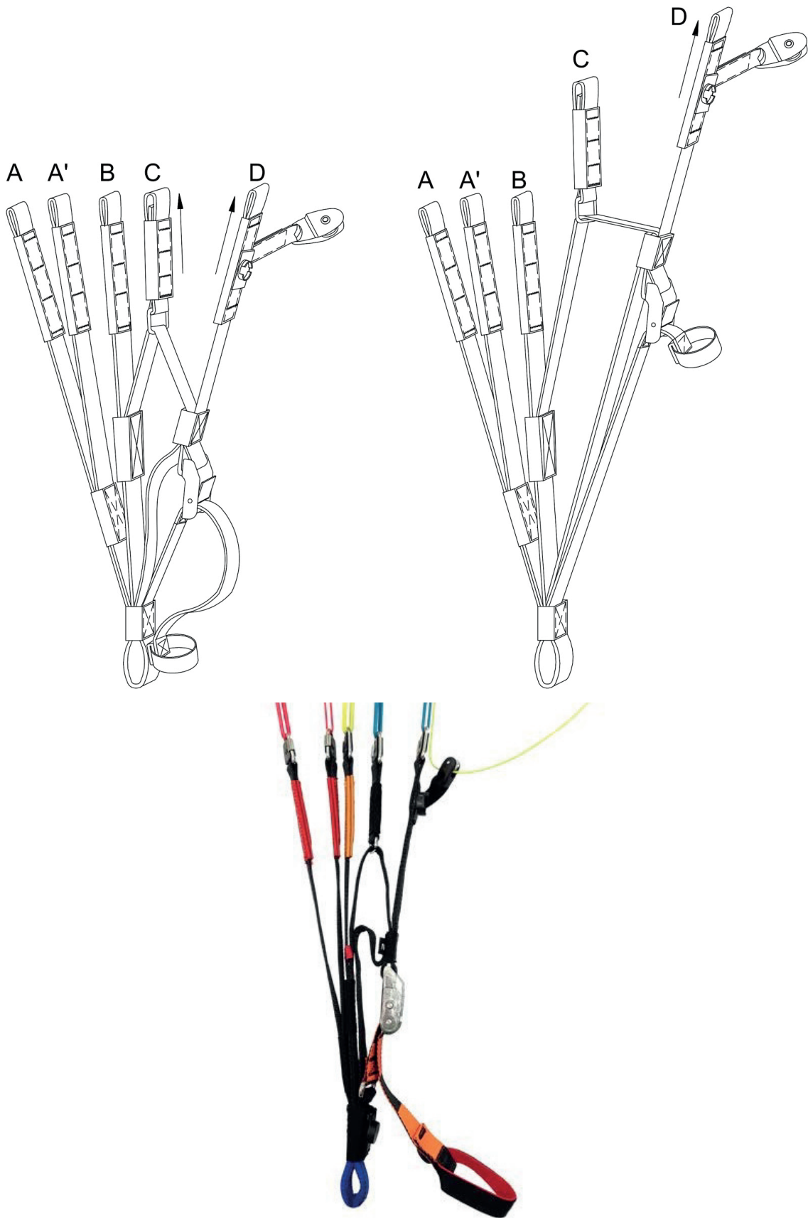
Figure: Optional Yeti Tandem 3 riser (12 mm Kevlar or 20 mm webbing version)
