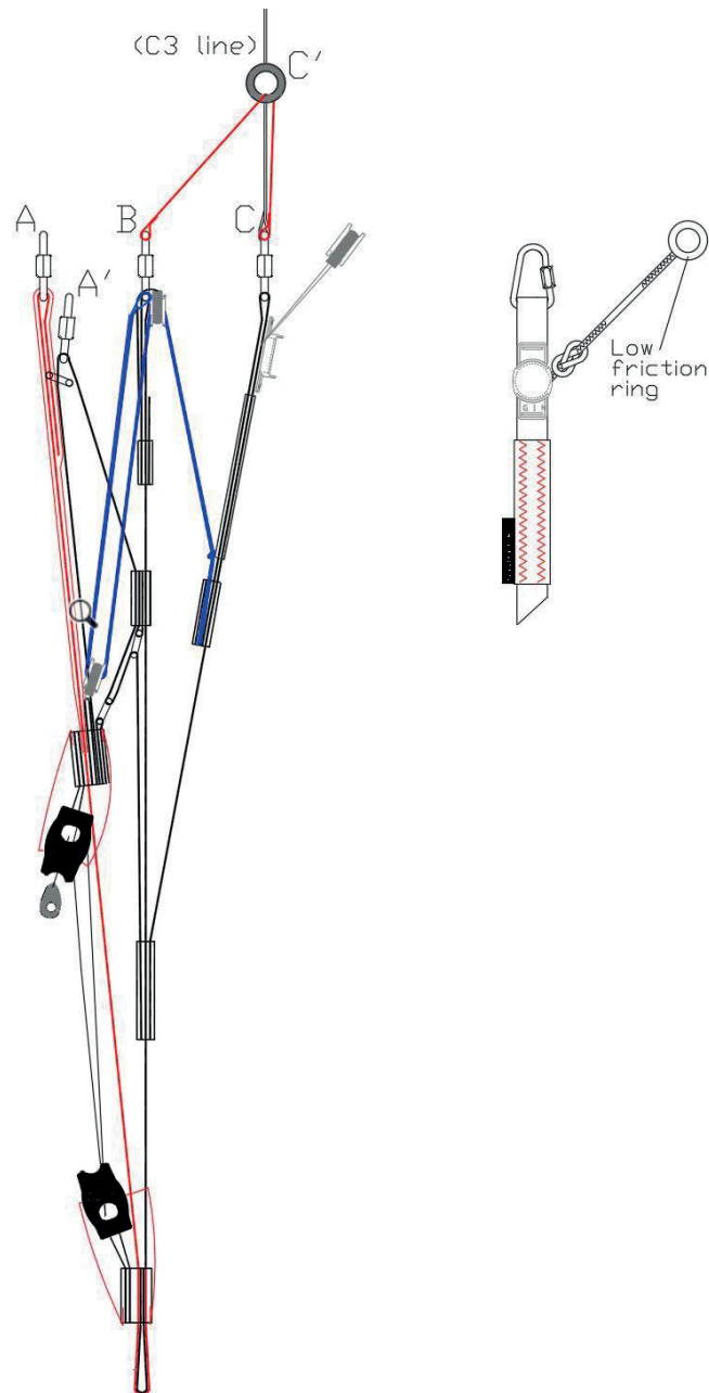
Figure: Camino riser (standard)
