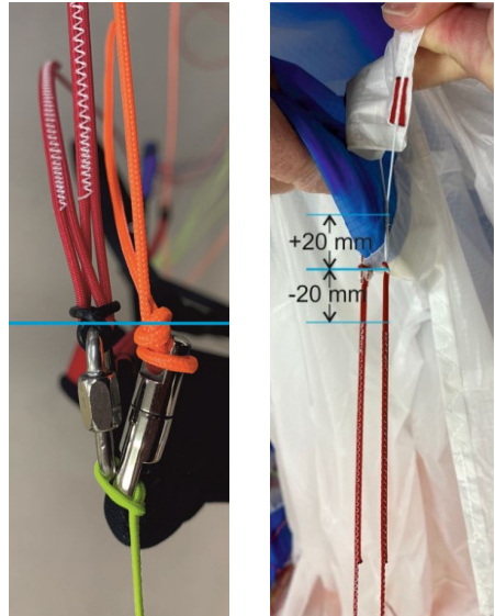
Fig. 10 Measuring points for the quick brake line check
