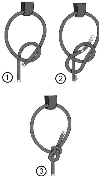
Fig. 5 Bowline knot
