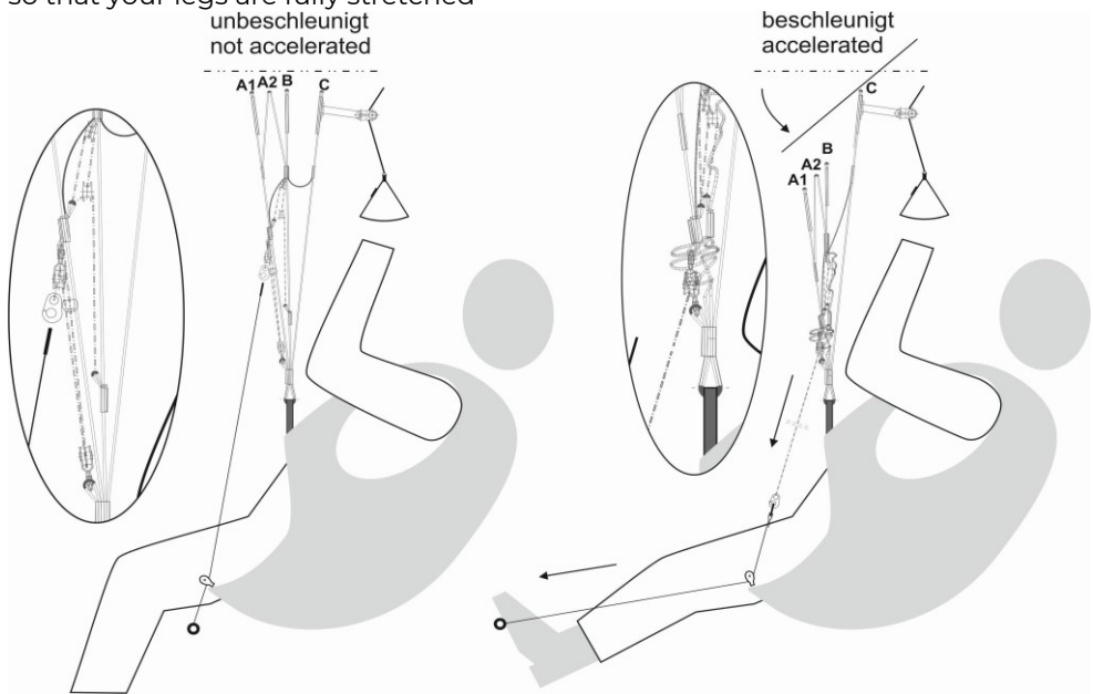
Fig. 7 How the ARCUS 2 RS speed system works
